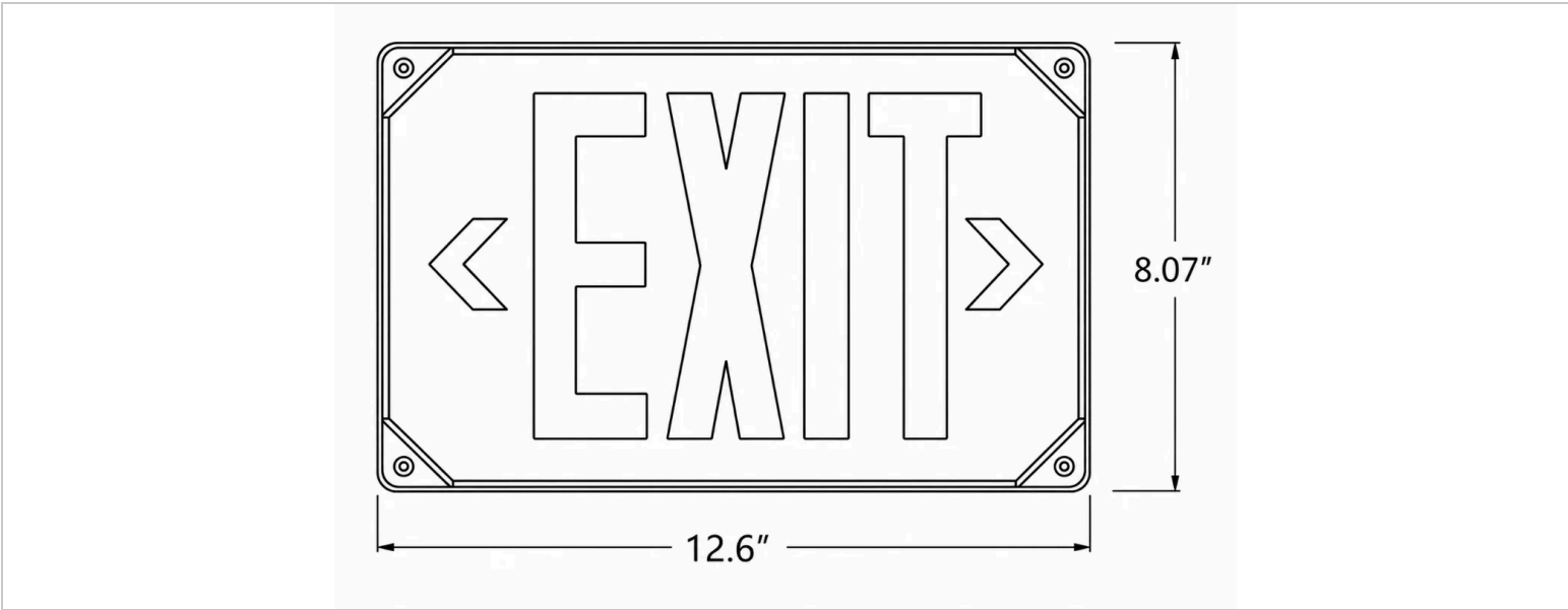
FIG. 02 · LINE DRAWING
