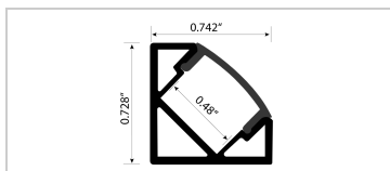
CORNER45 DLDT-S-CR45
